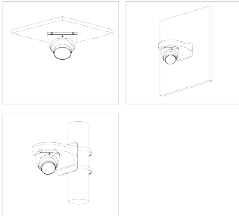
Figure 3-3 Installation method
